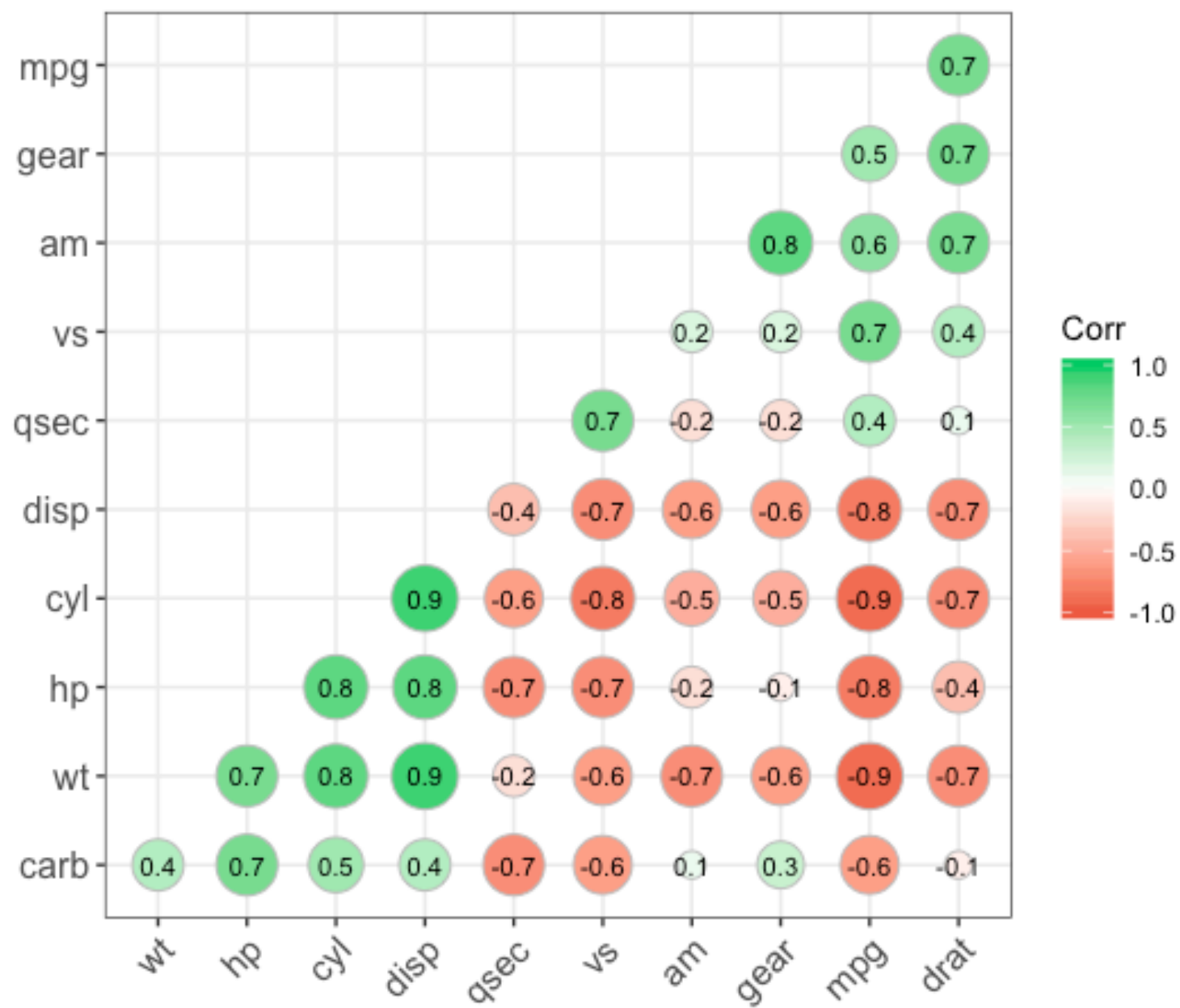
Correlogram of mtcars
